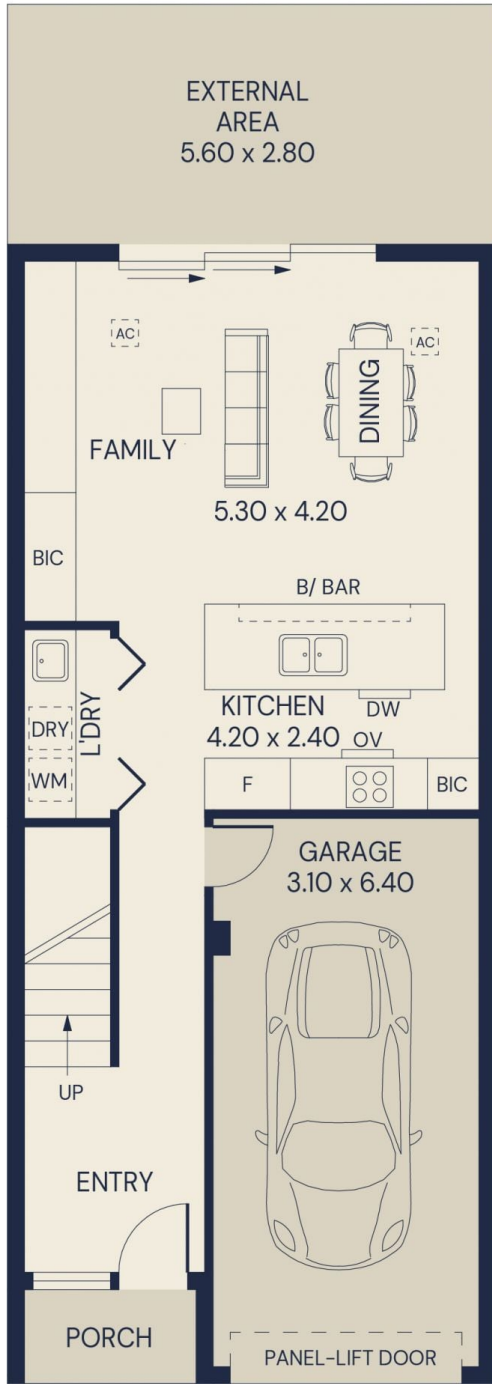
GROUND FLOOR
